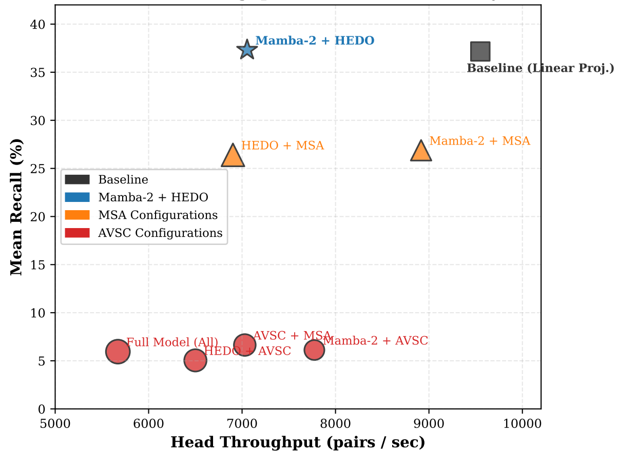
(a) Head Throughput vs. Retrieval Accuracy
